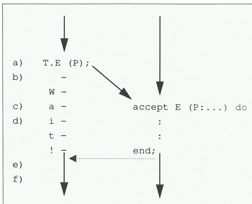
Figure 3: Task synchronization.
